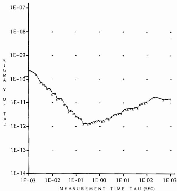
Sample \sigma_f(\tau) vs \tau plot generated by 5390A.
