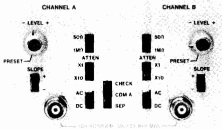
Figure 1. Input Switches
